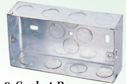
Switch & Socket Box Size: 1 Gang x 16mm & 25mm, 1 Gang x 35mm & 47mm, 2 Gang x 25mm & 35mm, Duel Box x 35mm
